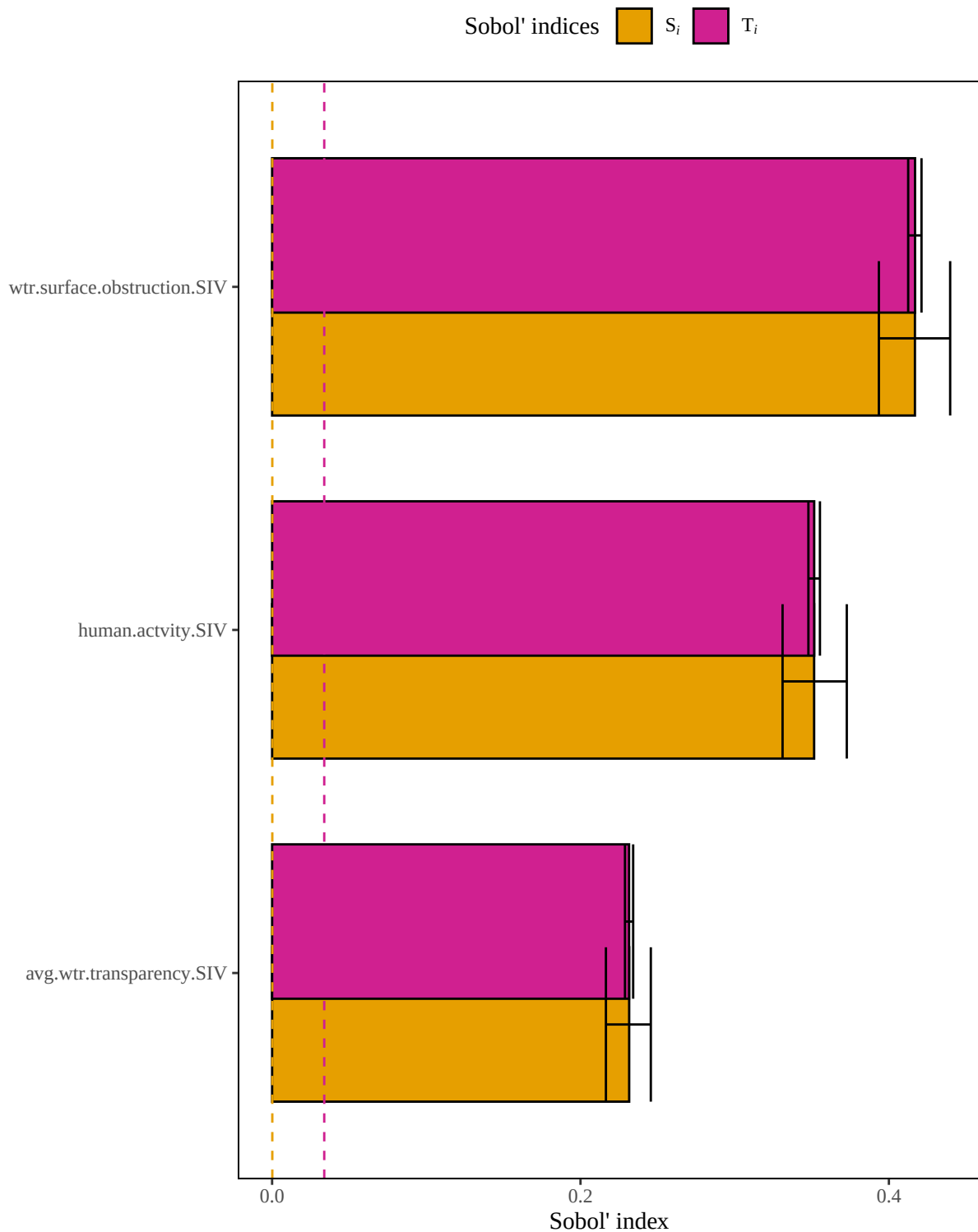
Figure 4. Results of a sensitivity analysis for the ospreyRiv model based on an arithmetic mean structure. Dashed lines represent baseline numerical approximation error for S_i and T_i ( i.e. , dummy variables).
